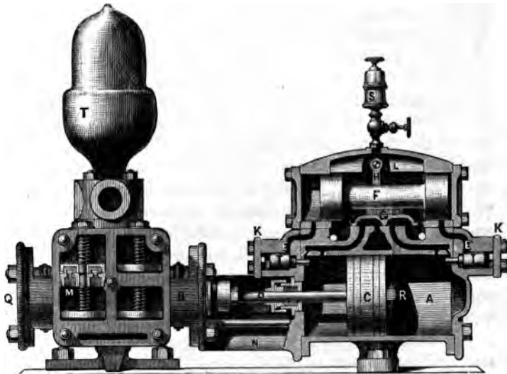
Fig. 102.—Steam-Pump.
